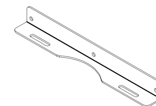
ISOMETRIC VIEW OF GROUND CONNECTION
