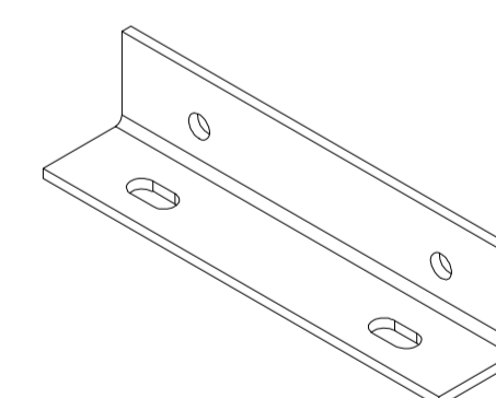
ISOMETRIC VIEW OF GROUND CONNECTION
